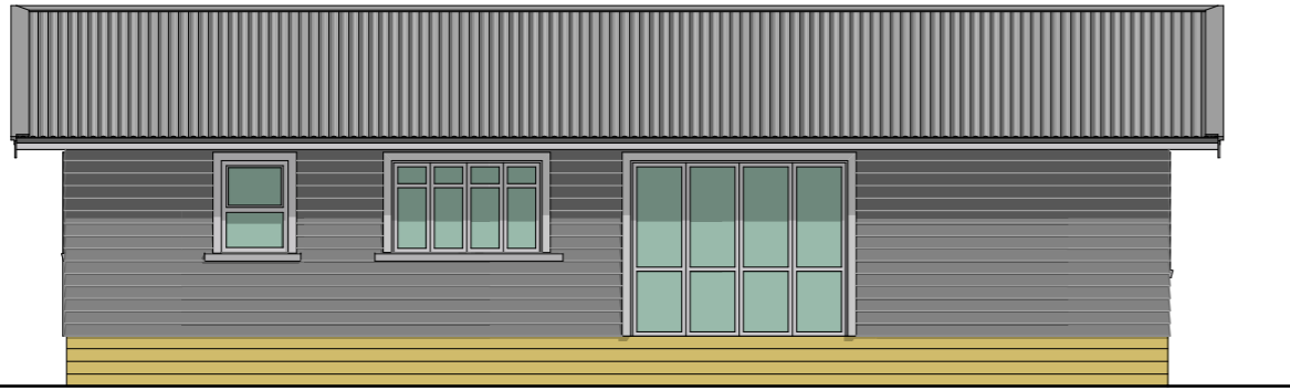
Proposed Elevation One Scale: 1:100
