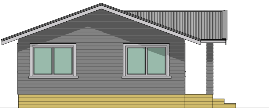
Proposed Elevation Four Scale: 1:100
