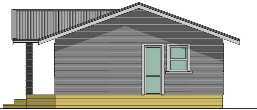
Proposed Elevation Two Scale: 1:100
