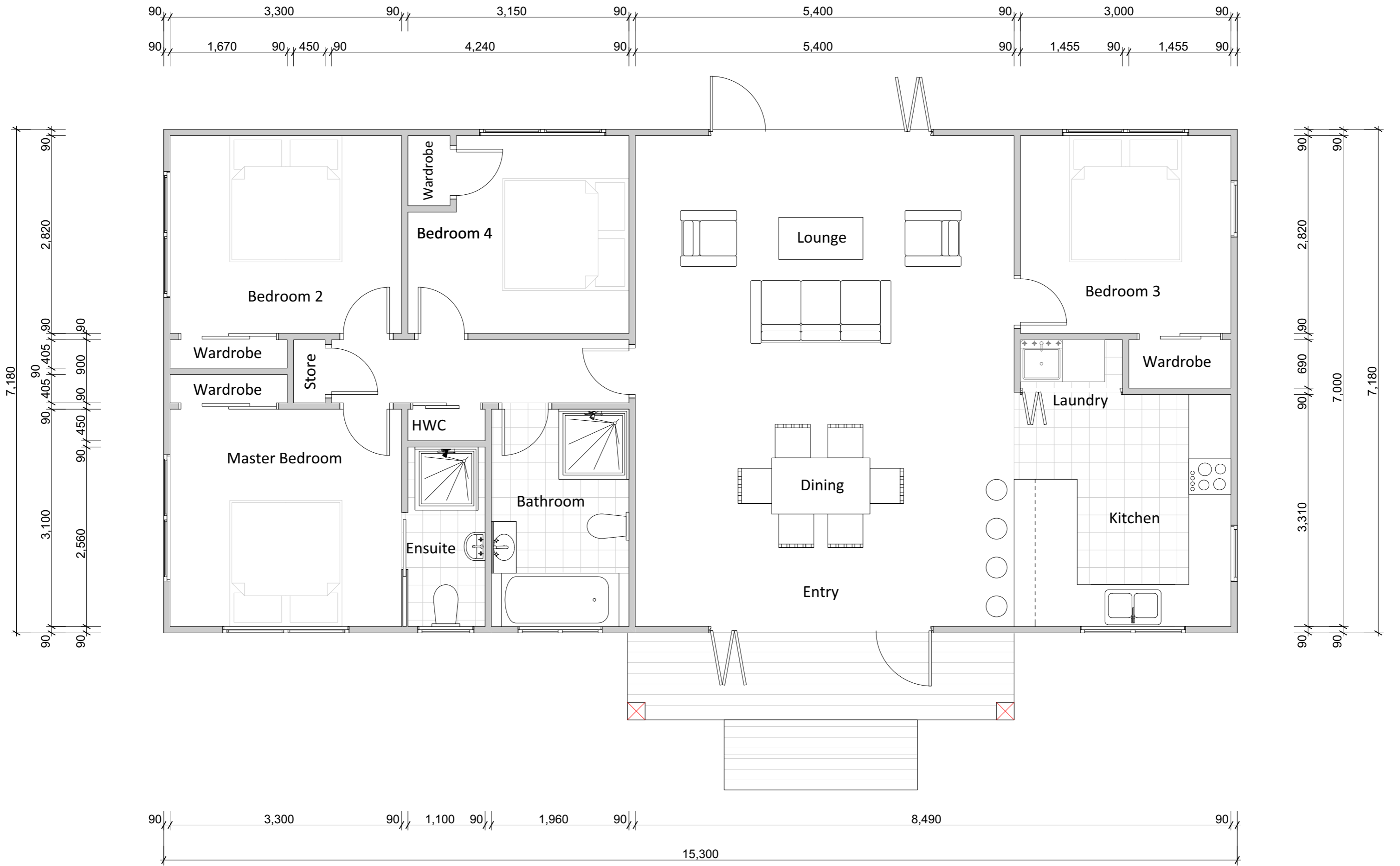
Proposed Floor Plan Scale: 1:50 (110m 2 )
