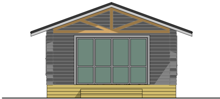
Proposed Elevation Two Scale: 1:100
