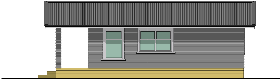
Proposed Elevation One Scale: 1:100
