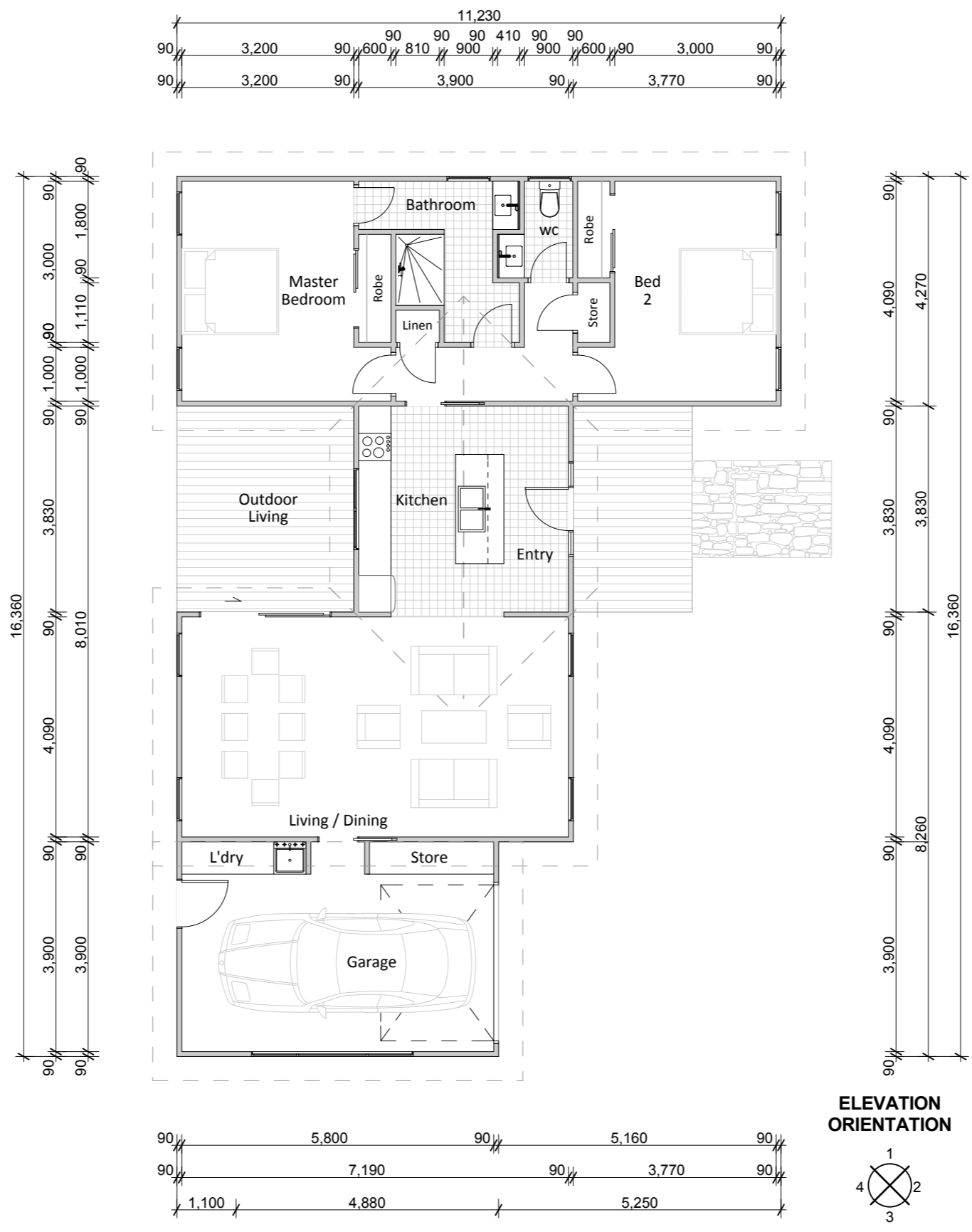
Proposed Floor Plan Scale 1:100 ( 119m2 )
